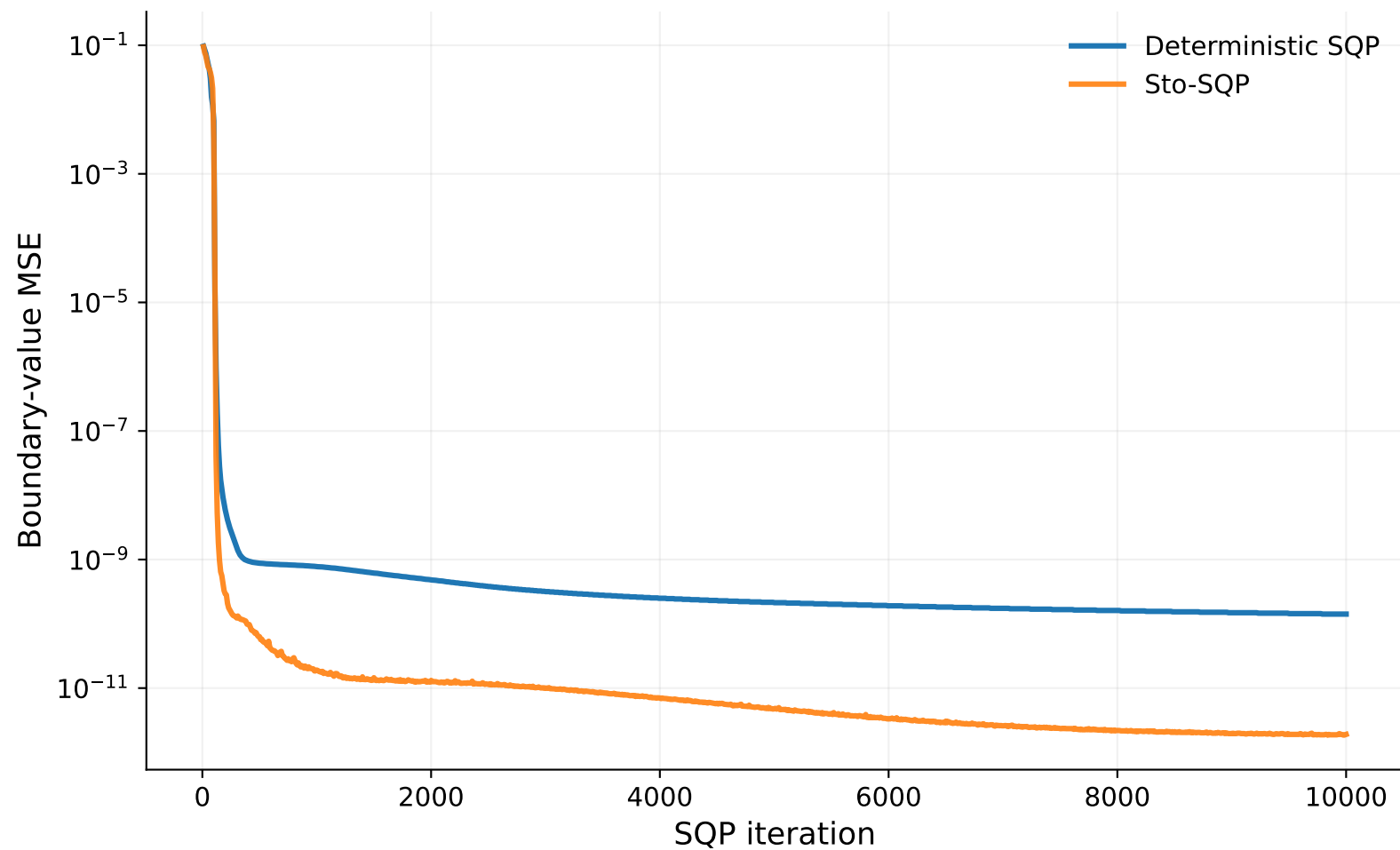
Burgers equation: boundary-value MSE — full trajectory
