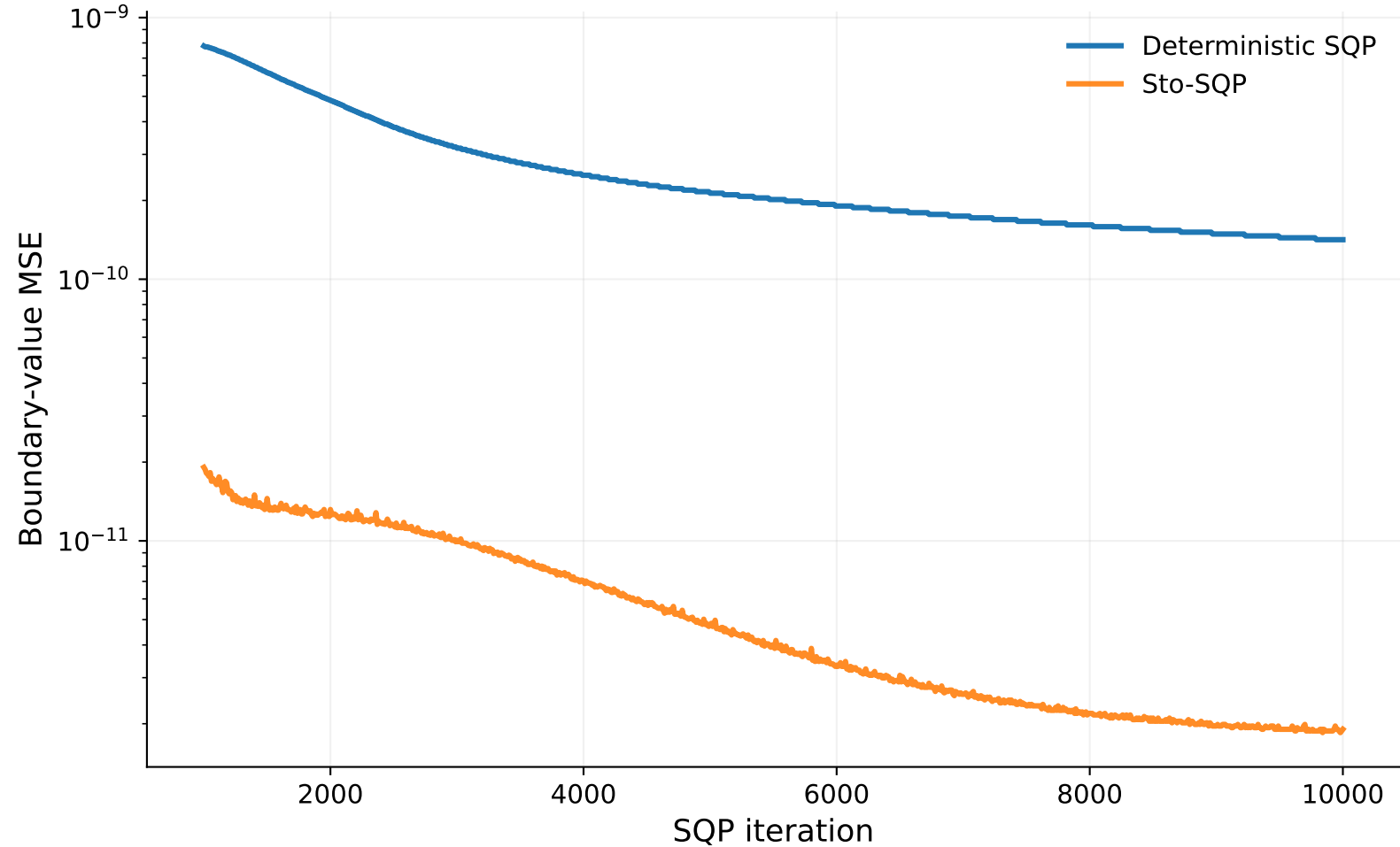
Burgers equation: boundary-value MSE — zoom: iter \geq 1000
